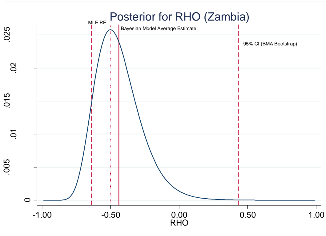
Figure 1 Bayesian Model Averaging Posterior for RHO Zambia 2007 (Men)
